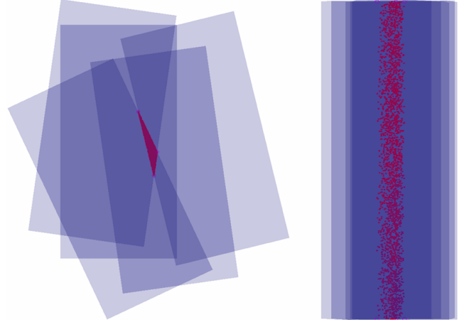
Fig. 3. Intersection of five instances of a TSR. Left : x-y view. Right : y-z view. The red points are sampled within the polytope of intersection using rejection sampling.
