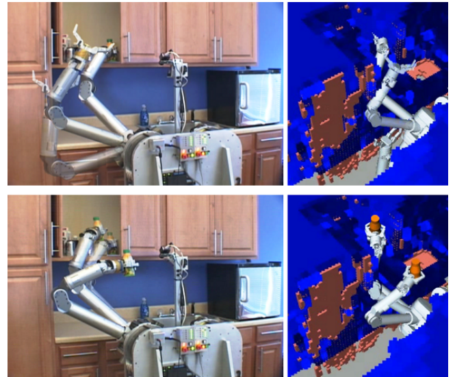
Fig. 7. Time-lapse images from the execution of two paths planned by GradientT-RRT with uncertain workspace occupancy. The blue areas in the robot’s world model (right) represent the probability of occupancy of a cell, with light blue being less occupied and dark blue being more occupied.
