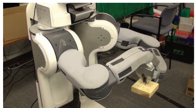
Figure 17. The PR2 executing the peg-insertion learning-assessment benchmark.
