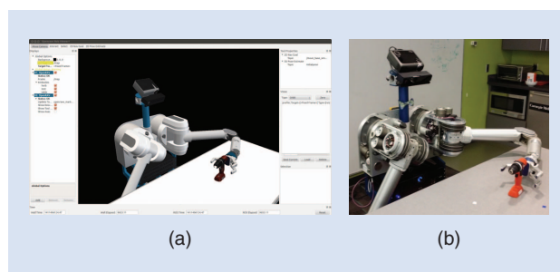
Figure 11. (a) The screen-capture from the OpenRAVE simulation and planning environment showing the HERB robot [34] planning a grasp of the power drill object in the set. (b) The actual grasp being executed by the robot on the physical object.
