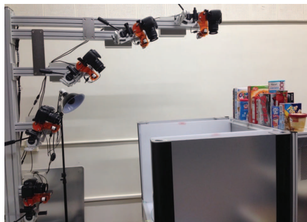
Figure 9. The BigBIRD object-scanning rig: the box contains a computer-controlled turntable.
