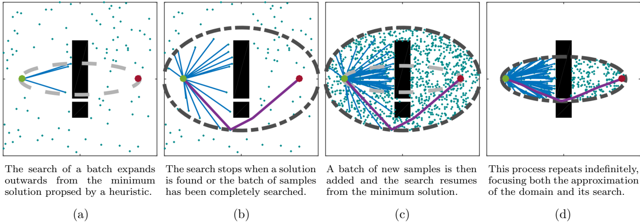
Figure 2. A simple example of the ordered sampling-based search performed by BIT*. The start and goal states are shown in green and red, respectively, while the current solution is highlighted in purple. The set of states that can provide a better solution (the informed set) is shown as a dark grey dashed line, while the progress of the current batch is shown as a light grey dashed line illustrating the informed set that the current edge would define. Fig. (a) shows the growing search of the first batch of samples, and (b) shows the first search ending when a solution is found. Note that ordering the search finds a solution without considering any states outside the informed set it defines. Fig. (c) shows the search continuing after pruning the representation and increasing its accuracy with a new batch of samples while (d) shows this second search ending when an improved solution is found.
