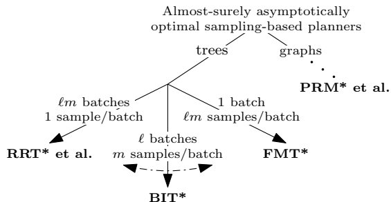
Figure 3. A simplified taxonomy of almost-surely asymptotically optimal sampling-based planners that demonstrates the relationship between RRT*, FMT*, and BIT*. When using a batch size of a single sample, BIT* is a version of RRT*. When using a single batch consisting of multiple-samples, BIT* is a version of FMT*.
