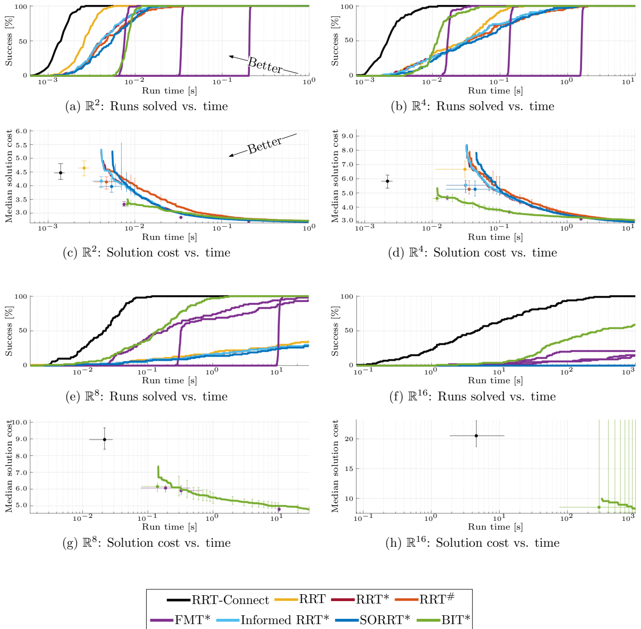
Figure 7. Planner performance versus time for the problem illustrated in Fig. 6a. Each planner was run 100 different times in \mathbb{R}^2 , \mathbb{R}^4 , \mathbb{R}^8 , and \mathbb{R}^{16} with run times limited to 1, 10, 30, and 1000 seconds, respectively. The percentage of trials solved is plotted versus run time for each planner and presented in (a), (b), (e), and (f). The median path length is plotted versus run time for each planner and presented in (c), (d), (g), and (h), with unsuccessful trials assigned infinite cost. The error bars denote a nonparametric 99% confidence interval on the median. The results show that BIT* is competitive to other almost-surely asymptotically optimal planners in \mathbb{R}^2 and outperforms them in all other tested state dimensions. Note the difficulty of solving this problem in \mathbb{R}^8 and \mathbb{R}^{16} in the available time.
