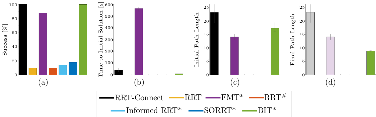
Figure 14. Results from 50, 600 second trials on the two-armed HERB planning problem shown in Fig. 13. The percent of solutions solved, (a), the median time to an initial solution, (b), the median initial path length, (c), and the median final path length, (d), are presented with 99% confidence intervals for each planner. Unsuccessful trials were assigned infinite time and cost. The inability of nonanytime planners (e.g., RRT, RRT-Connect, and FMT*) to use the remaining available time to improve their initial solution is denoted with diminished colour in (d), when present. BIT* is the only anytime planner to solve all 50 trials and does so in a time comparable to RRT-Connect. It focuses the search to the informed set once a solution is found and the resulting increasingly dense RGG allows it to find lower cost paths than all the other planners.
