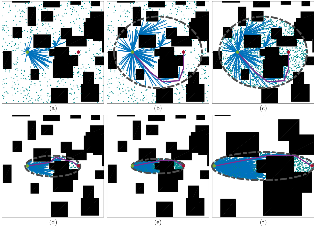
Figure 4. An example of how BIT* uses incremental techniques to efficiently search batches of samples in order of potential solution quality. The search starts with a batch of samples uniformly distributed in the planning domain. This batch is searched outward from the start in order of potential solution quality, (a). The search continues until the batch is exhausted or a solution is found that cannot be improved with the current samples, (b). New samples are then added to the informed set and incremental techniques are used to continue the search, (c)–(e). This results in an algorithm that performs an ordered anytime search that almost-surely asymptotically converges to the optimal solution, shown enlarged in (f). Note that BIT* orders all aspects of the search and never considers states in a batch that cannot provide the best solution (i.e., searches only inside the informed set defined by the eventual solution in the current graph).
