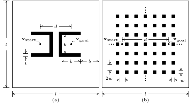
Figure 6. An illustration of the planning problems used in Sections 6.1.1 and 6.1.2. They are used to investigate algorithm performance on complex problems containing dual enclosures, (a), and many homotopy classes, (b), across state dimension. The problem dimensions in (a) were chosen to make the gaps symmetric, i.e., b = 0.6 , and l = 2.8 , for the chosen wall thickness, t = 0.1 . The width of the individual obstacles in (b) are chosen such that the start and goal states are 5 ‘columns’ apart in a problem domain of size l = 4 . For both problems, the distance between the start and goal, d , is 1.
