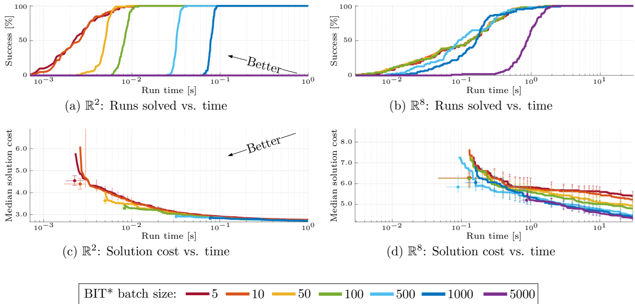
Figure 16. Planner performance versus time of BIT* with various batch sizes on the problem illustrated in Fig. 6a. Each configuration was run 100 different times in \mathbb{R}^2 and \mathbb{R}^8 with run times limited to 1 and 30 seconds, respectively. The percentage of trials solved is plotted versus run time and presented in (a) and (b). The median path length is plotted versus run time and presented in (c) and (d) with unsuccessful trials assigned infinite cost. The error bars denote a nonparametric 99% confidence interval on the median. It appears that decreasing the batch size decreases the median solution time towards a problem-specific threshold. The median initial solution time was the same in \mathbb{R}^2 for batch sizes of 5 and 10 samples but progressively higher for larger batches, (a). It was equivalent for batches of 5, 10, 50, and 100 samples in \mathbb{R}^4 (not shown) and for all tested batch sizes other than 5000 in \mathbb{R}^8 , (b). Decreasing the batch size also appears to decrease the rate of convergence towards the optimum, with the effect becoming more pronounced in higher state dimensions, (d). It is not clear how universal these relationships are between obstacle configurations.
