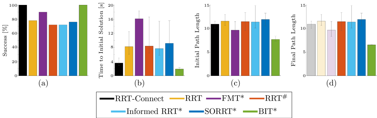
Figure 11. Results from 50, 20 second trials on the one-armed HERB planning problem shown in Fig. 10. The percent of solutions solved, (a), the median time to an initial solution, (b), the median initial path length, (c), and the median final path length, (d), are presented with 99% confidence intervals for each planner. Unsuccessful trials were assigned infinite time and cost. The inability of nonanytime planners (e.g., RRT, RRT-Connect, and FMT*) to use the remaining available time to improve their initial solution is denoted with diminished colour in (d), where present. BIT* is the only almost-surely asymptotically optimal planner to solve all 50 trials and does so in a time comparable to RRT-Connect. It also finds significantly lower cost paths than all the other planners.
