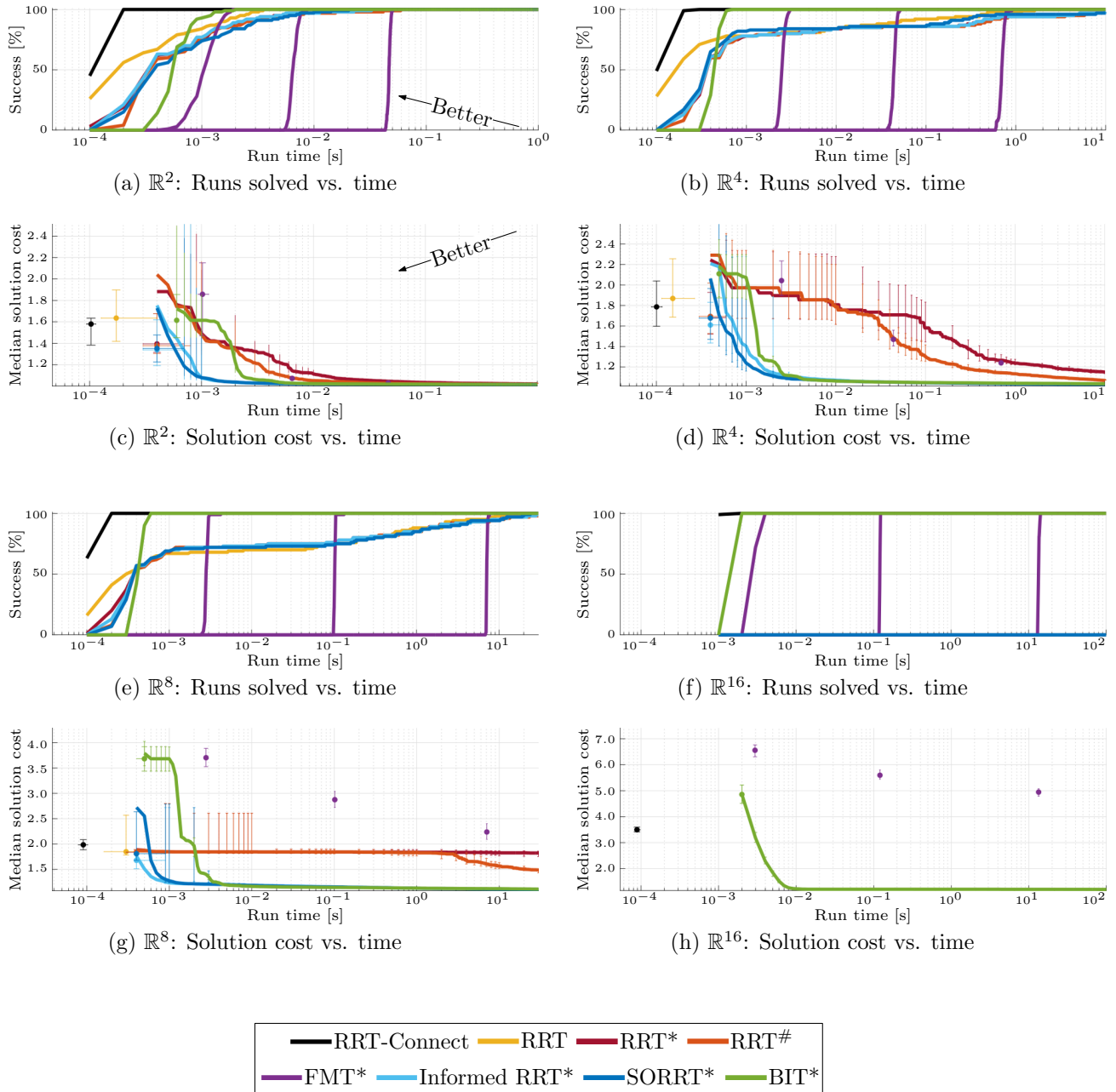
Figure 8. Planner performance versus time for the problem illustrated in Fig. 6b. Each planner was run 100 different times in \mathbb{R}^2 , \mathbb{R}^4 , \mathbb{R}^8 , and \mathbb{R}^{16} with run times limited to 1, 10, 30, and 100 seconds, respectively. The percentage of trials solved is plotted versus run time for each planner and presented in (a), (b), (e), and (f). The median path length is plotted versus run time for each planner and presented in (c), (d), (g), and (h), with unsuccessful trials assigned infinite cost. The error bars denote a nonparametric 99% confidence interval on the median. The results show that on this problem BIT* finds a solution to all trials faster than all tested planners other than RRT-Connect and outperforms other almost-surely asymptotically optimal planners in \mathbb{R}^{16} . Note that RRT*-based planners are not able to find solutions for this high state dimension in the time available.
