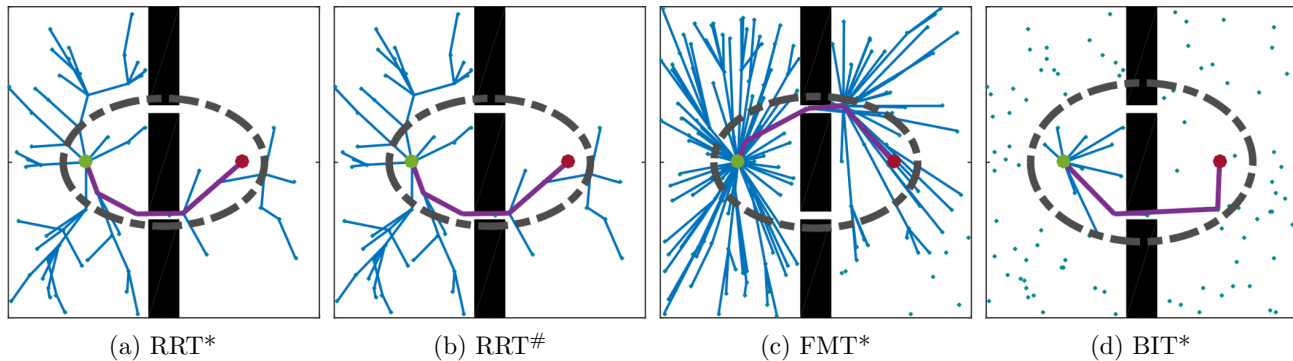
Figure 1. The relative efficiency of the searches performed by RRT* (a), RRT# (b), FMT* (c), and BIT* (d) as illustrated by their initial solution and its resulting informed set. Each planner was run until an initial solution was found and then stopped. The resulting set of states that could provide a better solution is shown as a dark-grey dashed line. Search outside this informed set is provably unnecessary for the solution found by each planner and illustrates the inefficiency of the initial search of RRT*, RRT#, and FMT*, (a)–(c). Note that RRT# finds an initial solution from the same samples as RRT* as the heuristics presented in Arslan and Tsiotras (2015) do not alter the search until a solution is found. Also note that by ordering its search on potential solution quality, BIT* does not consider any samples that cannot provide the best solution in its current approximation (i.e., batch of samples). The start and goal states of the problem are shown in green and red, respectively, while the graph built by the planner is shown in blue and the initial solution is highlighted in purple.
