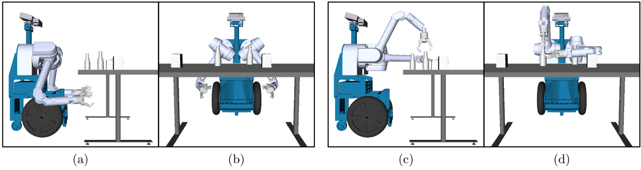
Figure 13. A two-armed motion planning problem for HERB in \mathbb{R}^{14} . Starting under the table, (a) and (b), HERB's arms must be moved in preparation for opening a bottle, (c) and (d).
