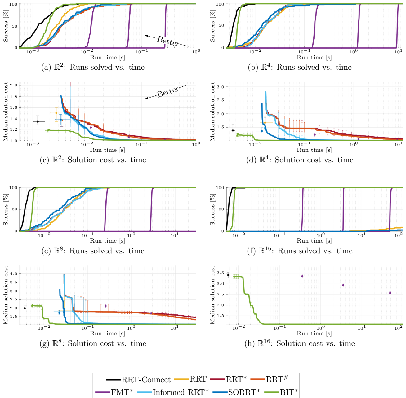
Figure 9. Planner performance versus time for a randomly generated problem. Each planner was run 100 different times in \mathbb{R}^2 , \mathbb{R}^4 , \mathbb{R}^8 , and \mathbb{R}^{16} with run times limited to 1, 10, 30, and 100 seconds, respectively. The percentage of trials solved is plotted versus run time for each planner and presented in (a), (b), (e), and (f). The median path length is plotted versus run time for each planner and presented in (c), (d), (g), and (h), with unsuccessful trials assigned infinite cost. The error bars denote a nonparametric 99% confidence interval on the median. The results show that BIT* outperforms other almost-surely asymptotically optimal planners in both ability to solve the problem and median solution cost. Note the increase in this difference with higher state dimension and the difficulty of solving the problem in \mathbb{R}^{16} in the available time with RRT*-based planners.
