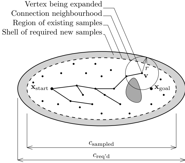
Figure 5. An illustration of just-in-time (JIT) sampling. Samples are generated only when they are necessary for the expansion of a vertex, \mathbf{v} , into the edge queue. This is accomplished while maintaining uniform sample density by an expanding informed set. The informed set is expanded by adding uniformly distributed samples in the prolate hyperspheroidal shell defined by the difference between the maximum heuristic value of the neighbourhood, c_{\text{req'd}} , and the currently sampled informed set, c_{\text{sampled}} .
