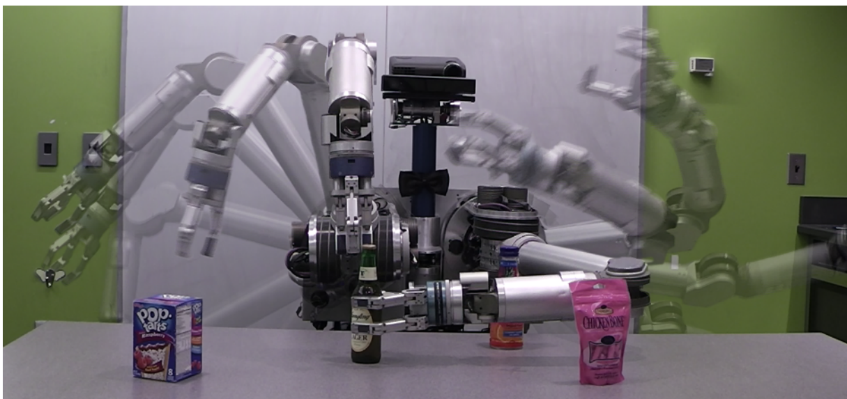
Figure 15. A composite figure of HERB executing a path found by BIT* on a two-armed planning problem similar to Fig. 13.
