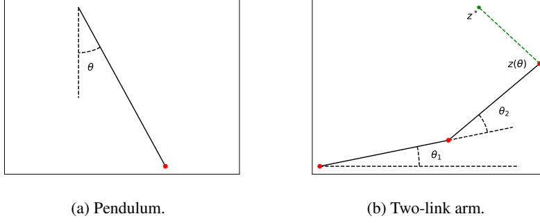
Figure 6: Control settings considered.
