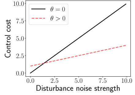
Figure 2: Expected behavior of the risk-sensitive controllers for increasing disturbance noise.
