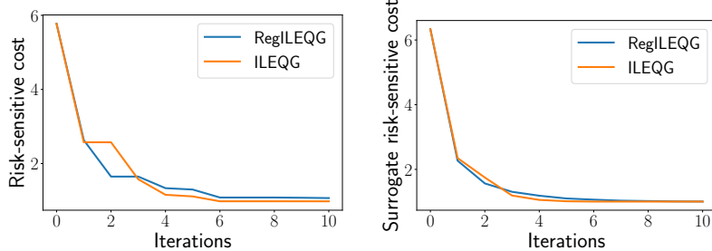
Figure 3: Convergence of iterative linearized methods, RegILEQG and ILEQG, on the pendulum problem.
