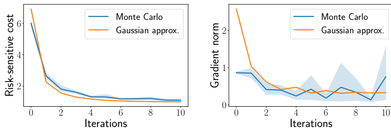
Figure 4: Risk-sensitive and gradient approximations.
