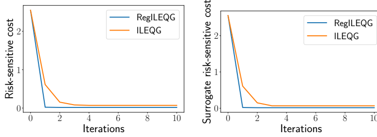
Figure 7: Convergence of iterative linearized methods, RegILEQG and ILEQG, on the two-link arm problem.
