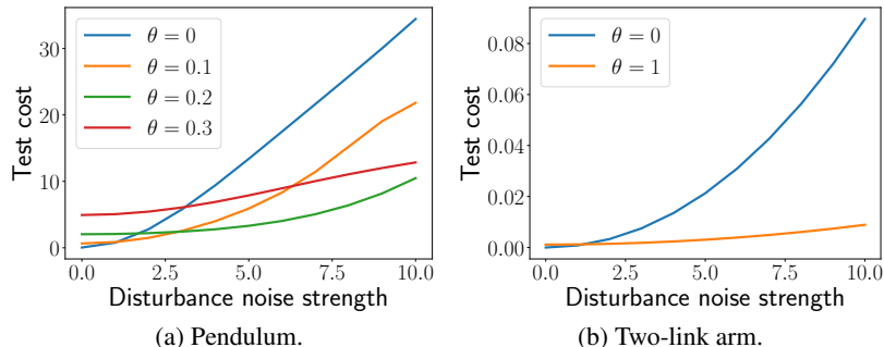
Figure 5: Robustness of controllers against disturbance noise.
