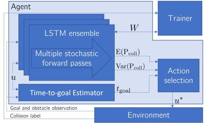
Fig. 2: System architecture
