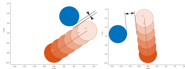
(a) Obstacle in training, confident (b) Obstacle in test, cautious
